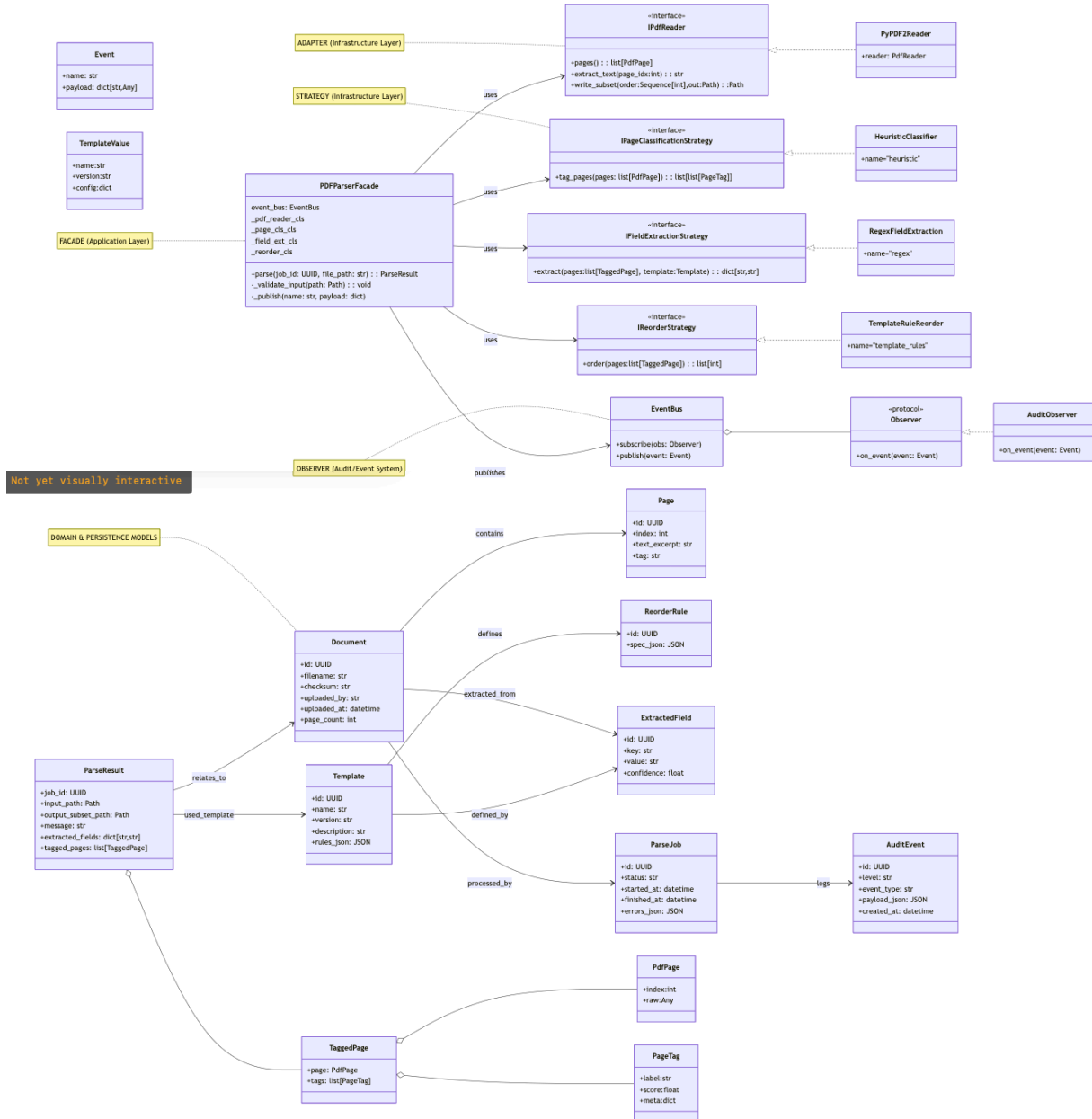
FIGURE 5 : UML Class Diagram
